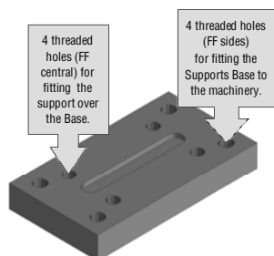
Supports Base art.BD LXR...FF series with threaded holes. Normally used for mobile support with nut.
