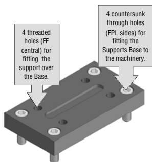
Supports Base art.BD LXR...FPL with countersunk through holes at sides. Normally used for fixed supports with bearings and DXC with bush.
